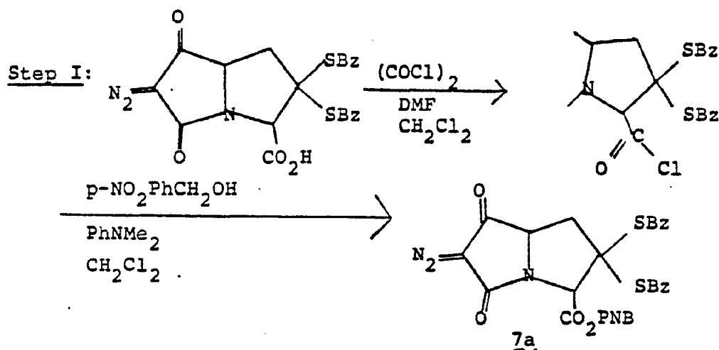
2-Carbo-p-nitrobenzyloxy-3,3-dithiobenzyl-7-diazo-6,8-dioxo-1-azabicyclo[3.3.0]octane
