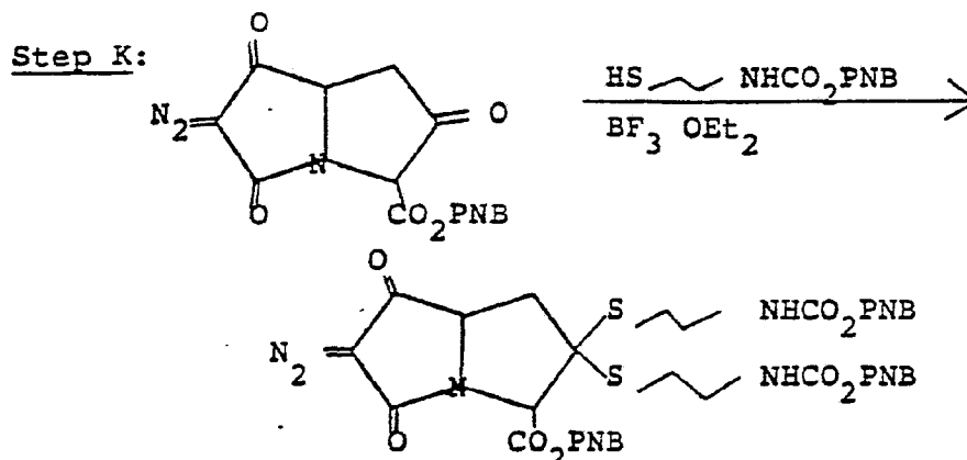
2-Carbo-p-nitrobenzyloxy-3,3-bis(N-carbo-p-nitrobenzyloxy-β-aminoethylthio)-7-diazo-6,8-dioxo-1-azabicyclo[3.3.0]octane
