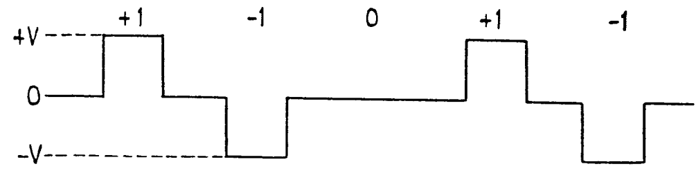
(a) TERNARY LINE SIGNAL
