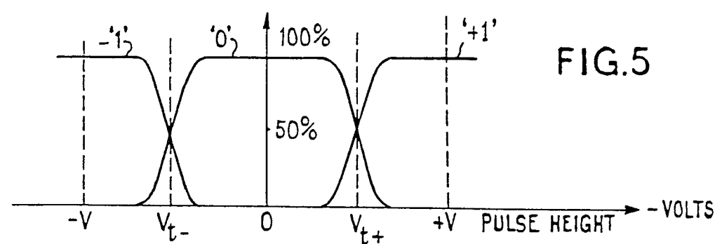
(b) PROBABILITY OF STATE DETECTED IN RECEIVER VERSUS MAGNITUDE OF TRANSMITTED PULSE
