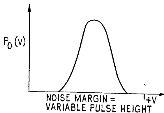
(a) pdf OF NOISE MARGIN FOR '0'
