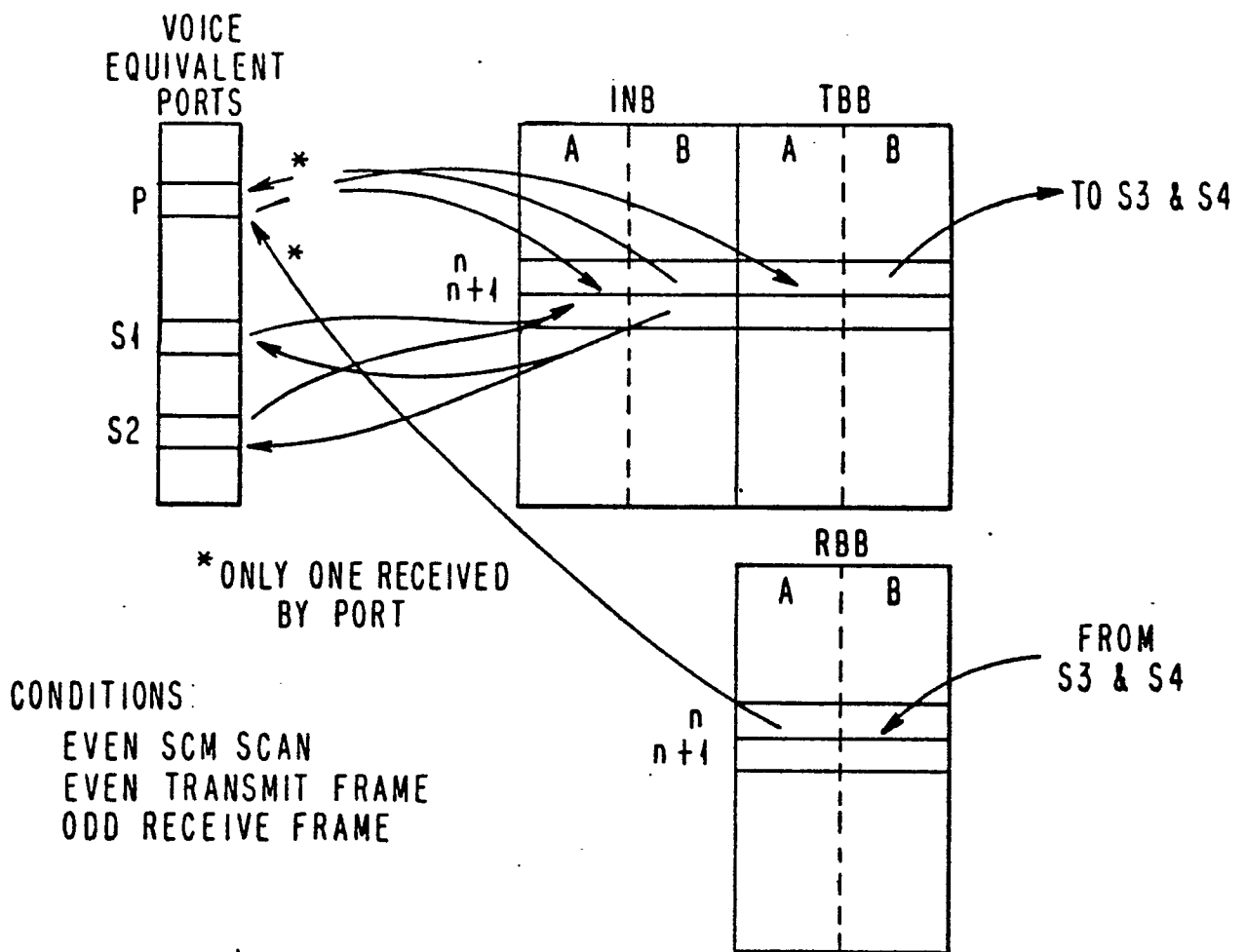
FIG.30 PORTS COMMUNICATING IN A CONFERENCE CONNECTION
