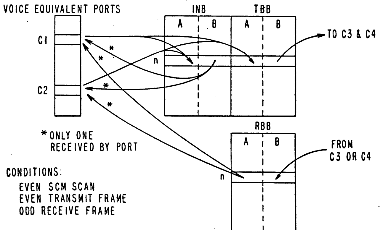
FIG.30 PORTS COMMUNICATING IN A CONFERENCE CONNECTION
