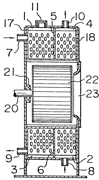
FIG. 2 PRIOR ART
