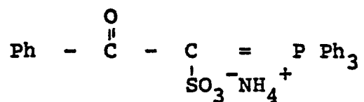
(Compound 14)
