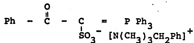
(Compound 15)
