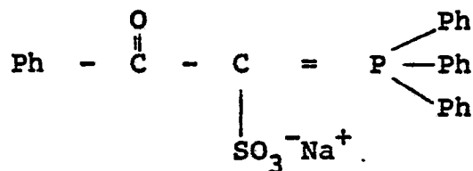
(Compound 8)
