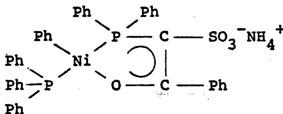
(Compound 11)
