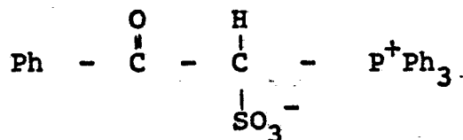
(Compound 7)
