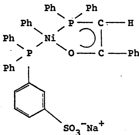
(Compound 3)
