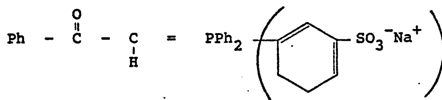
(Compound 5)
