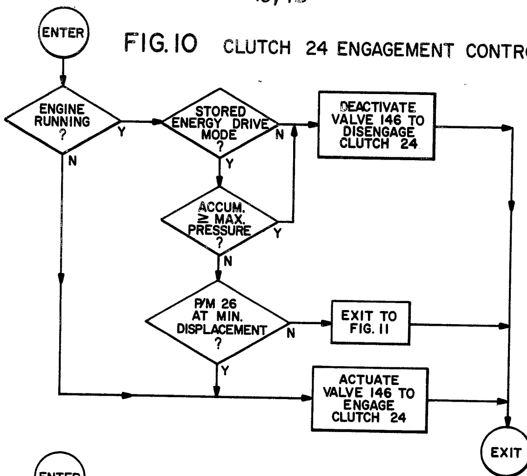
P/M 26 DISPLACEMENT CONTROL
