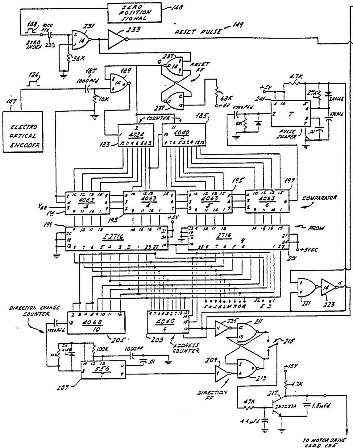
FIG. 6. FIRST SECTION
