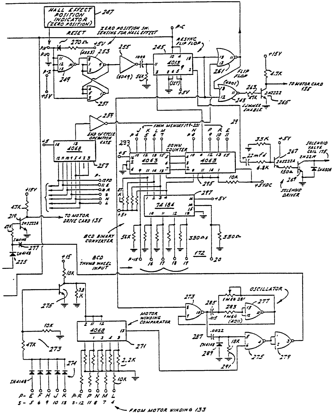
FIG. 6. SECOND SECTION
