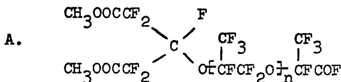
Chemical Shifts \delta ppm
