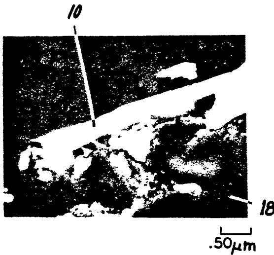
FIG. 2a DRILLED
