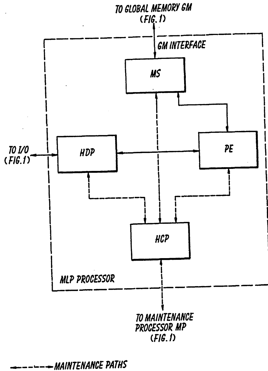
FIG. 2 MLP PROCESSOR
