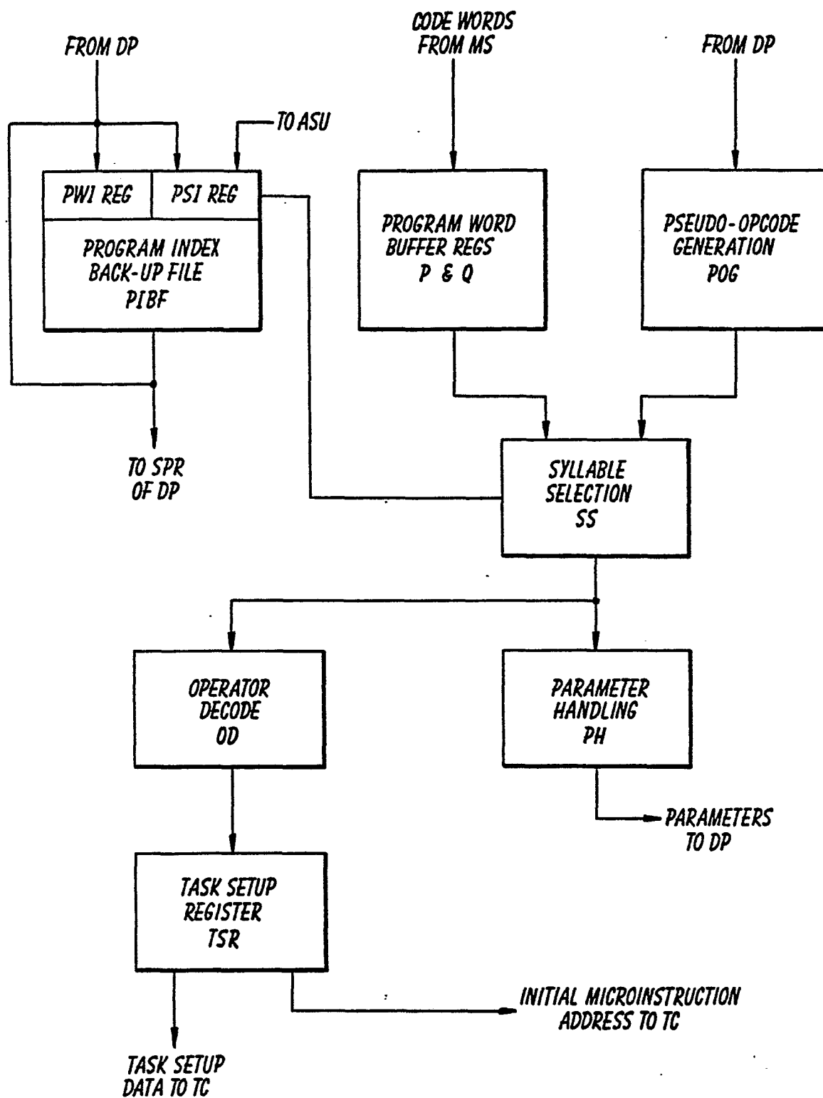
FIG. 9 PROGRAM CONTROLLER PC
