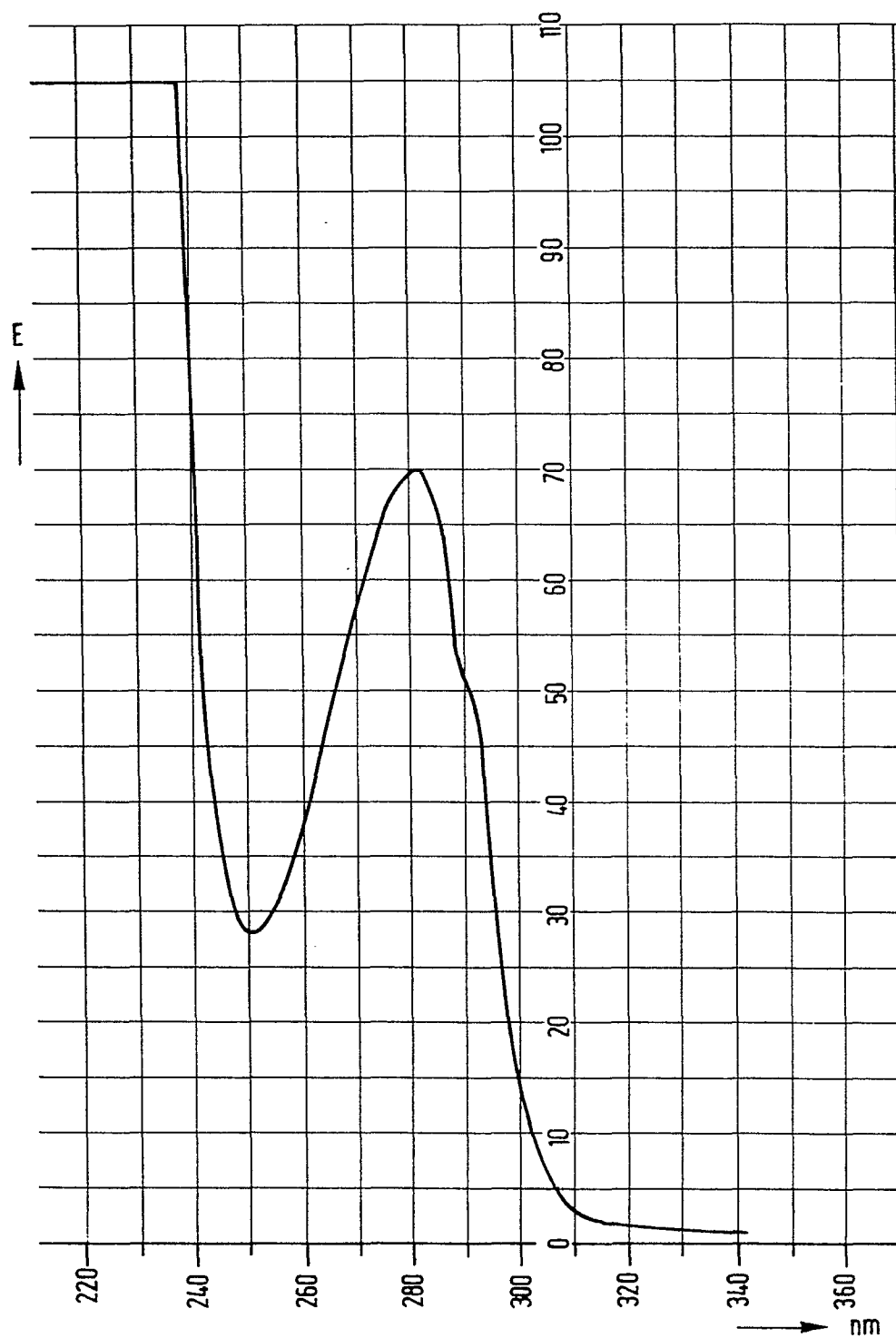
ABSORPTION SPECTRUM OF THE GRANULOCYTO-BLASTOGEN IN WATER AT 20°C. EXTINCTION SCALE (0-100)
