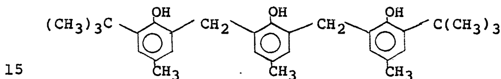
2,6-Bis(2'-hydroxy-3'-t-butyl-5'-methyl-benzyl)-4-methyl phenol
