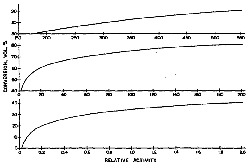
FIG. 1 MAT. CONVERSION VS. RELATIVE ACTIVITY REFERENCE CATALYST CONVERSION: 75% DAVISON FEEDSTOCK
