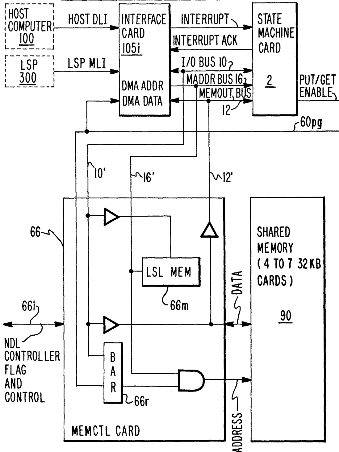
FIG. 7. EXTERNAL BUS LOGIC BLOCK DIAGRAM.
