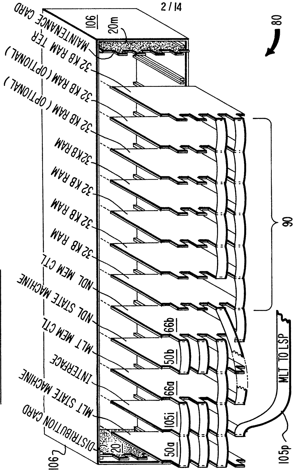
FIG.1B. NETWORK SUPPORT PROCESSOR.
