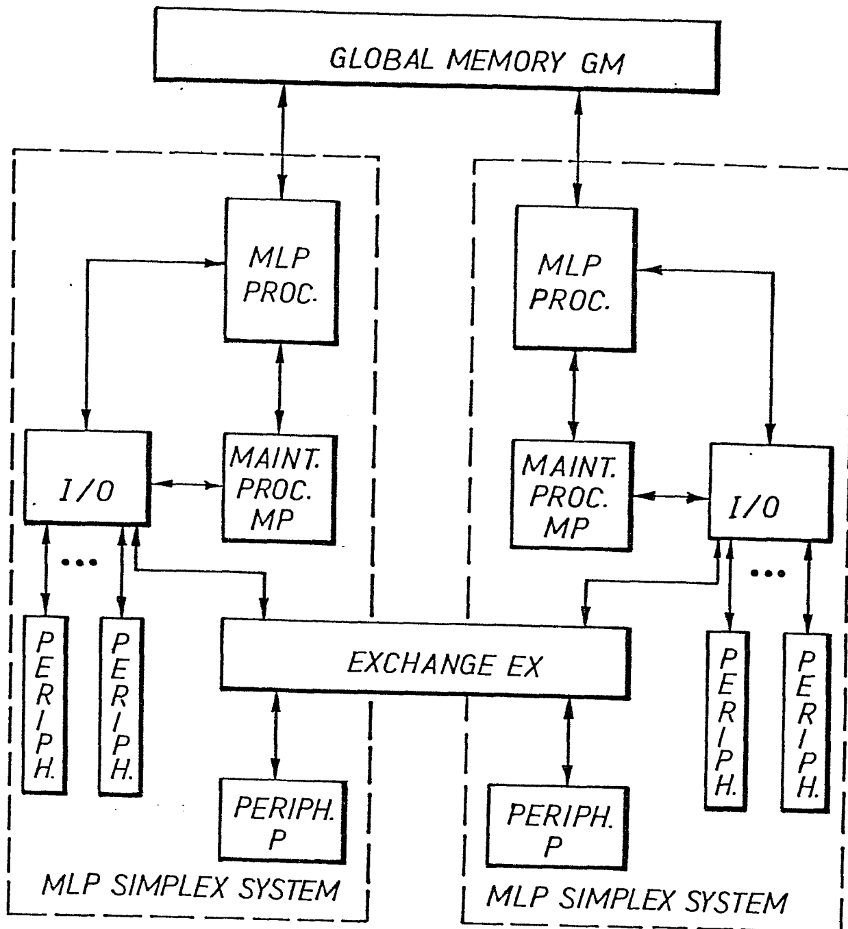
FIG. 1 OVERALL-SYSTEM
