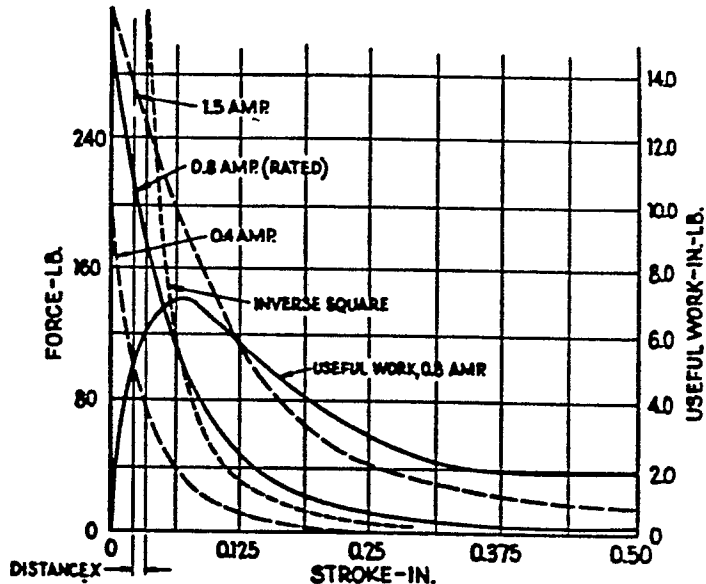
FLAT-FACED PLUNGER MAGNET AND ITS FORCE-STROKE CURVES
