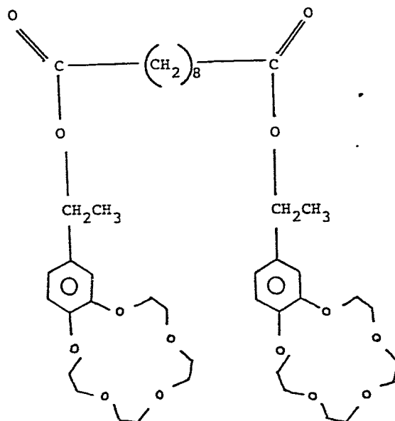
Bis-(4'-ethylbenzo-15-Crown-5) Sebacate
