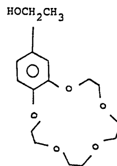
4'-hydroxyethylbenzo-15-Crown-5
