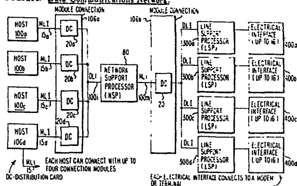
FIG. 1A. Data Communications Network
