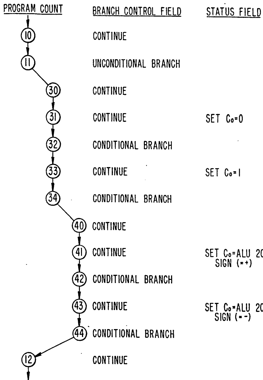
FIG. 24 UNCONDITIONAL/CONDITIONAL BRANCH CONTROL
