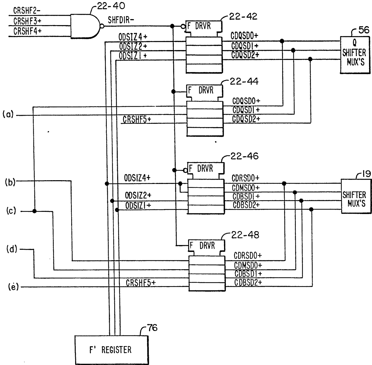
SHIFT DISTANCE CONTROL LOGIC 22-12
