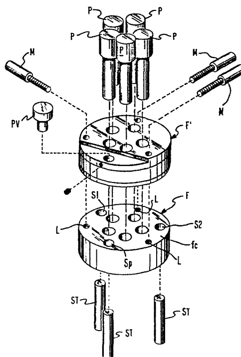
FIG.1. FLOATING LAPPING FIXTURE
