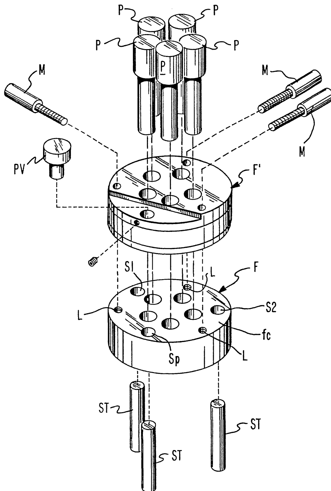
FIG.1. FLOATING LAPPING FIXTURE.
