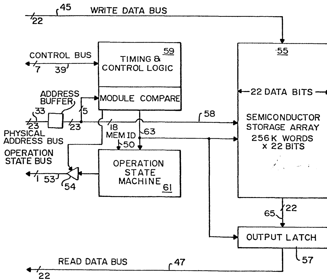
FIG. 2 SEMICONDUCTOR MEMORY MODULE
