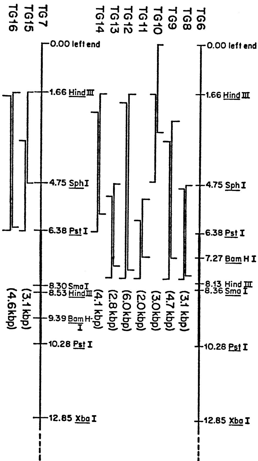
Fig.4--Hybrid Phages TG6 and TG7 and Deletion Mutants
