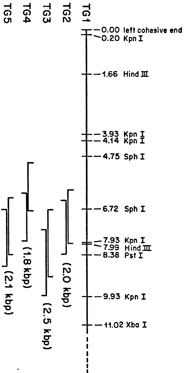
Fig. 3 - Deletion Mutants of Phage TG1
