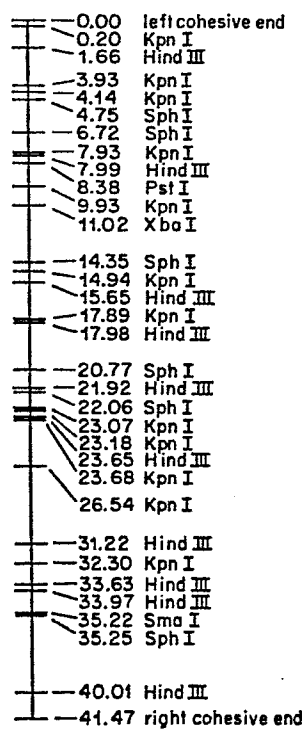
Fig. 2 – Restriction Map of Phage TG1
