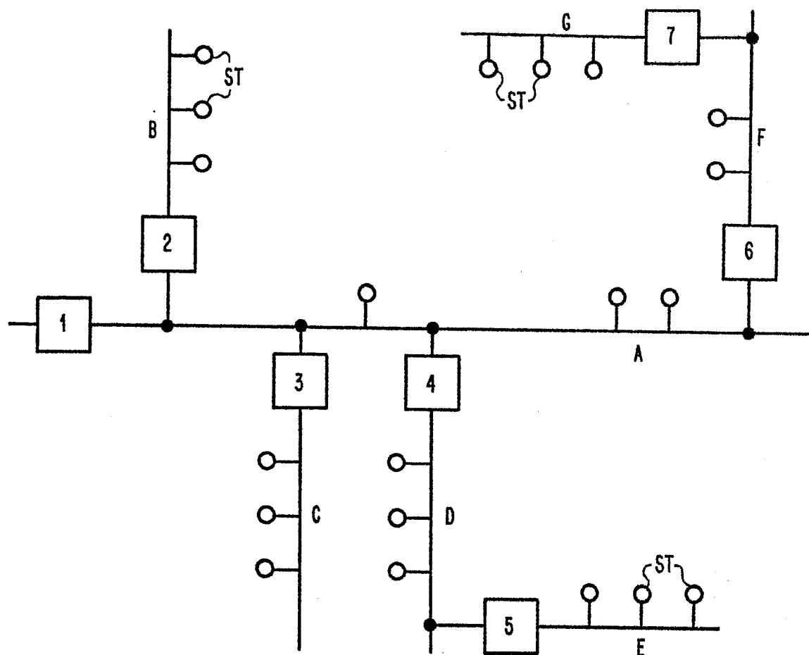
FIG. 1 NETWORK CONFIGURATION
