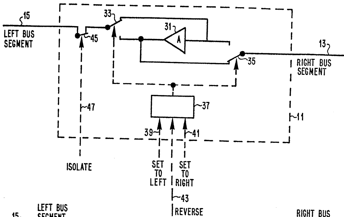
FIG. 3 SWITCH AND REPEATER UNIT
