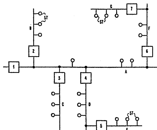
FIG. 1 NETWORK CONFIGURATION
