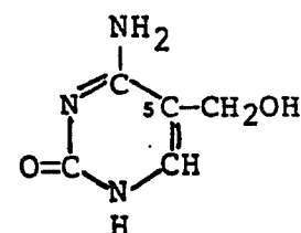
5-Hydroxymethylcytosine
