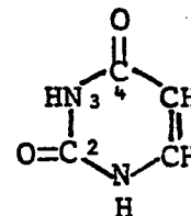
Uracil (2,4-dioxypyrimidine)
