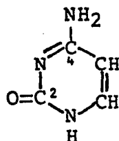
Cytosine (2-oxy-4-aminopyrimidine)
