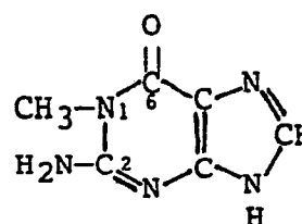
1-Methylguanine
