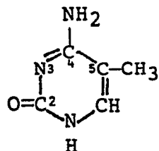
5-Methylcytosine
