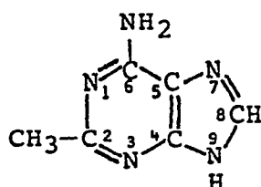
2-Methyladenine
