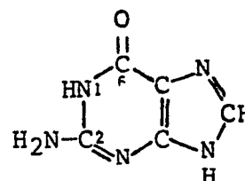
Guanine (2-amino-6-oxypurine)
