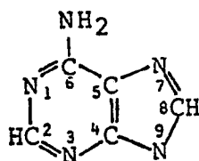
Adenine (6-aminopurine)
