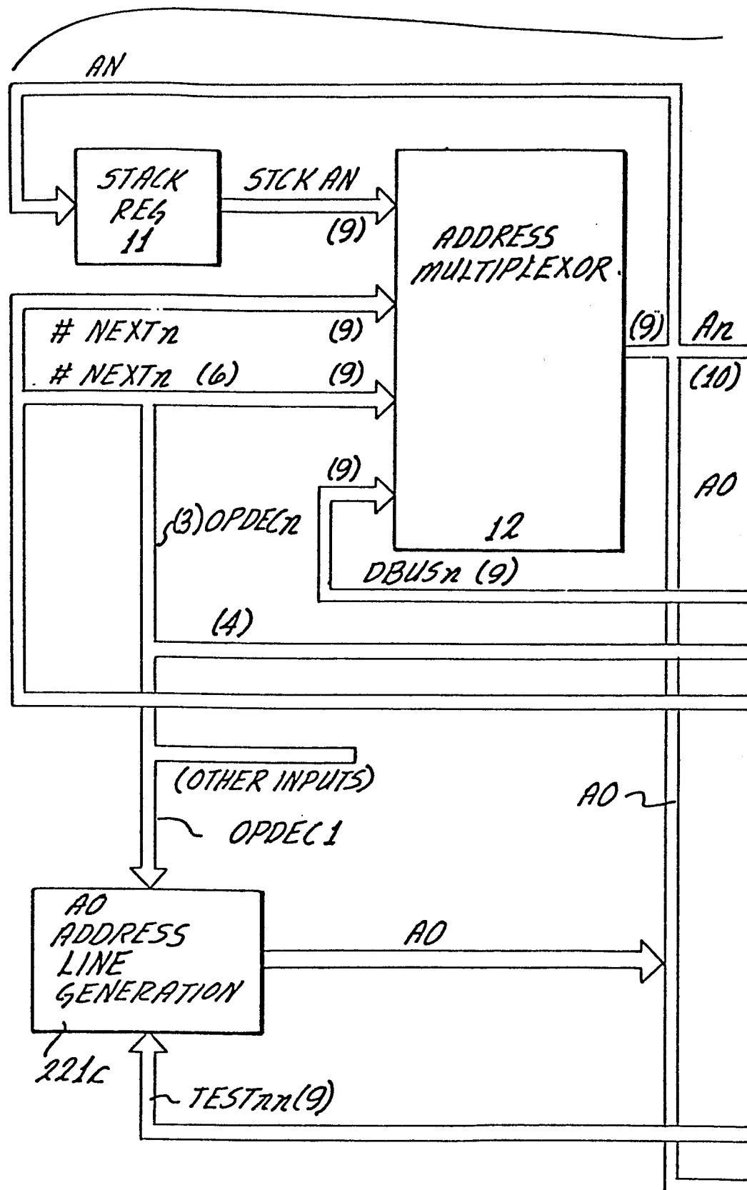
FIG. 5A-1: BLOCK DIAGRAM FOR ON-LINE OPERATION
