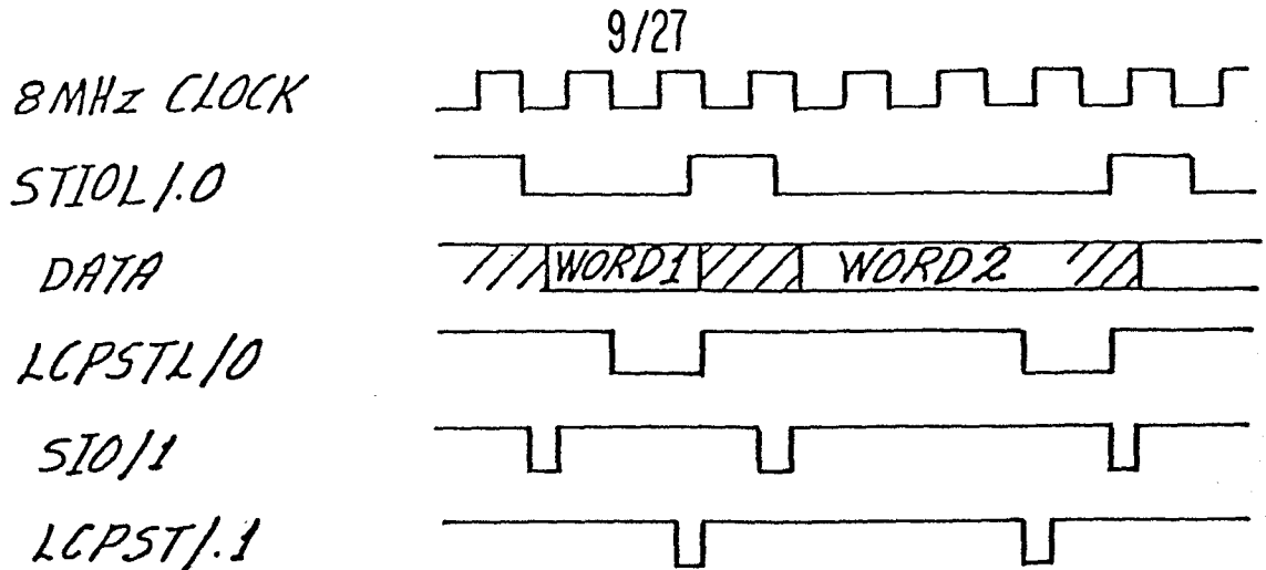
Fig. 4E DATA TRANSFER TIMING DIAGRAM (DISTRIBUTION CARD-DLP INTERFACE)
