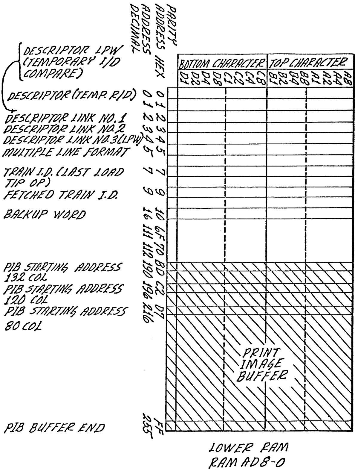
FIG. 5C-1 MEMORY USAGE KEY : 5C-1 5C-2
