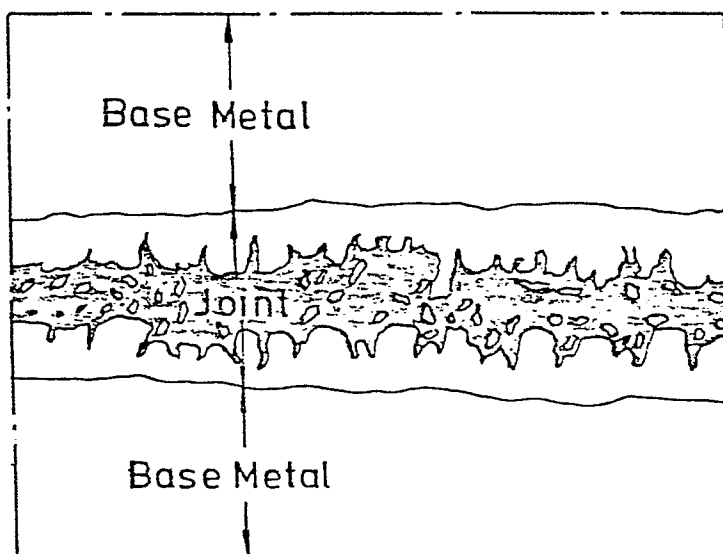
Photomicrograph of AISI 316 stainless steel joint brazed with Sample No. 2 alloy of the present invention (Magnification 400 X).
