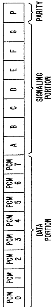
FIG. 6 16-BIT DATA WORD
