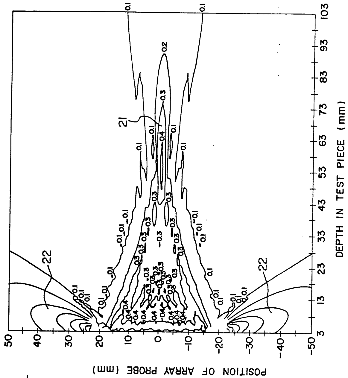
FIG. 2 PRIOR ART
