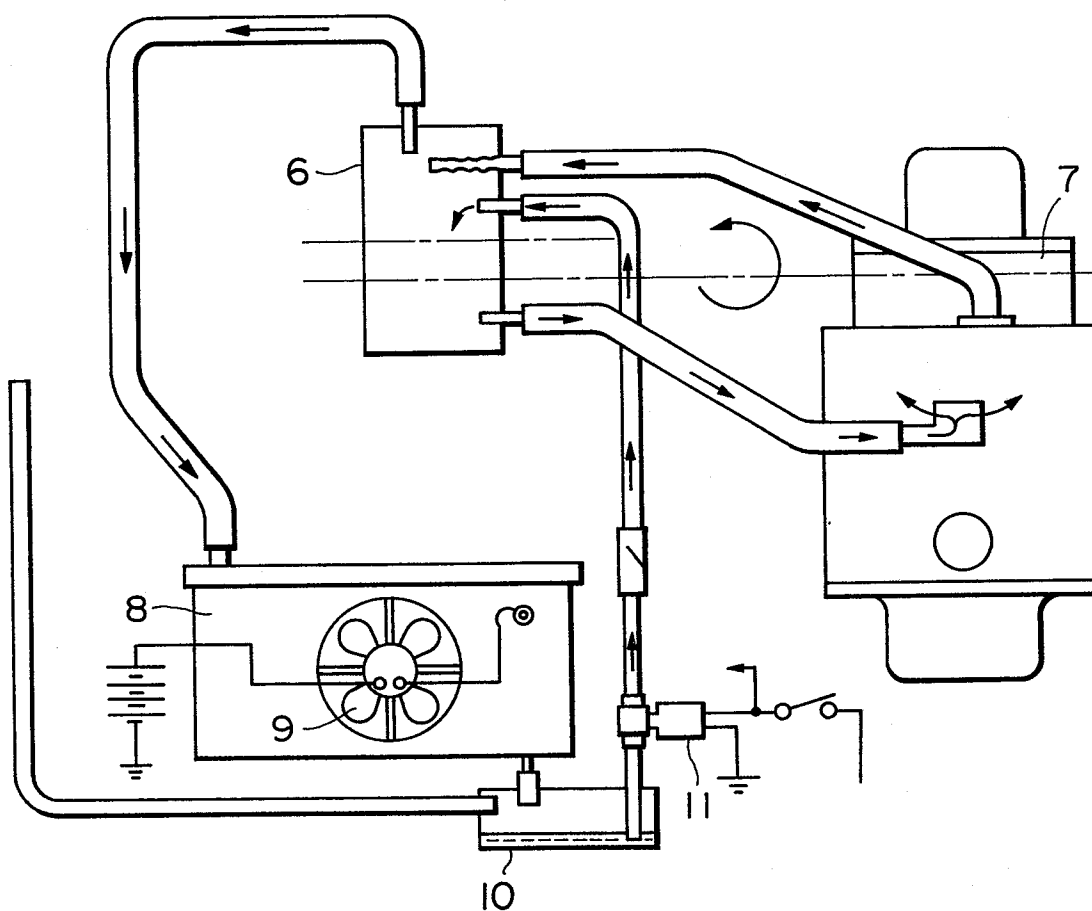
FIG.2 (PRIOR ART)
