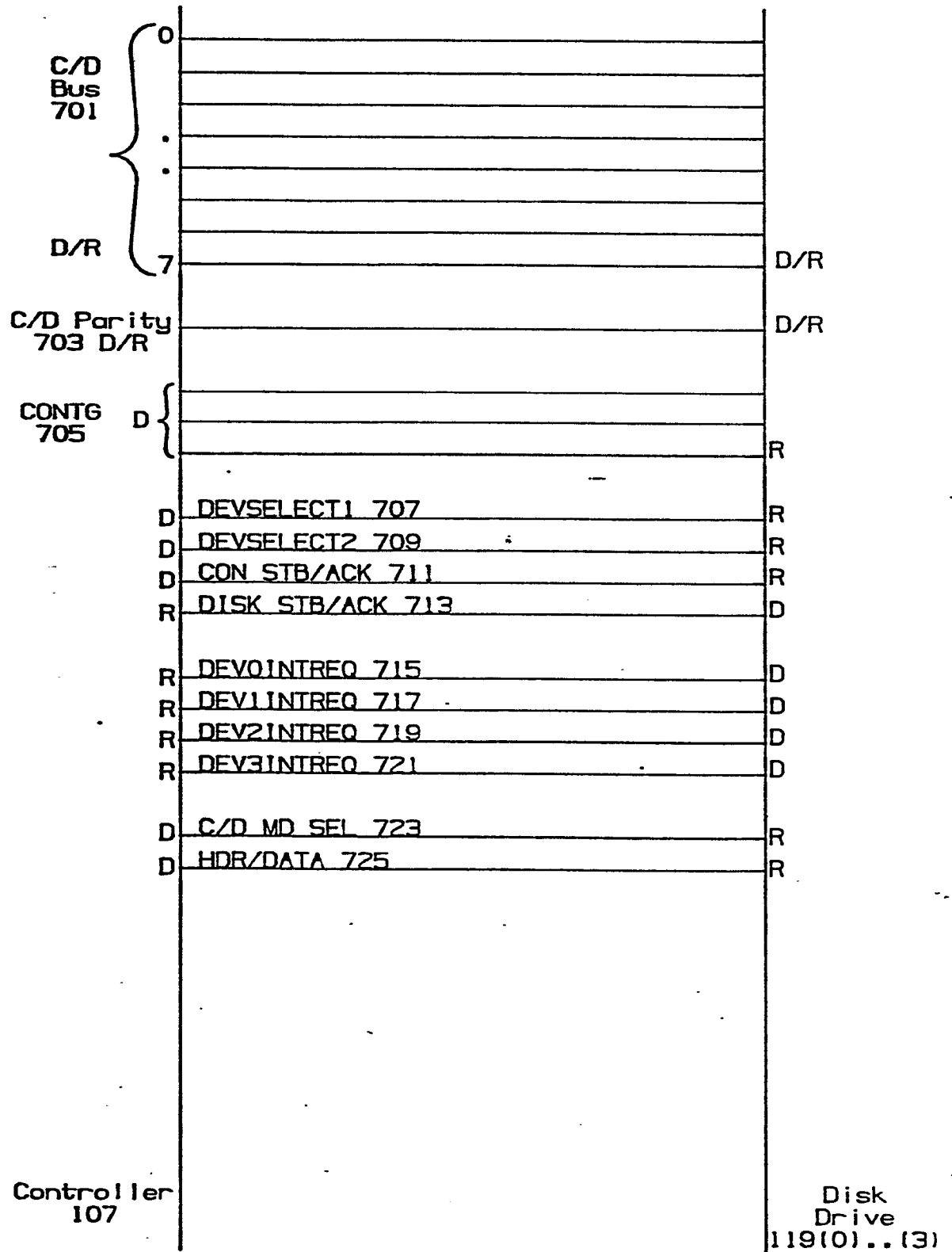
Fig.7: Controller-Disk Bus 127 Detail
