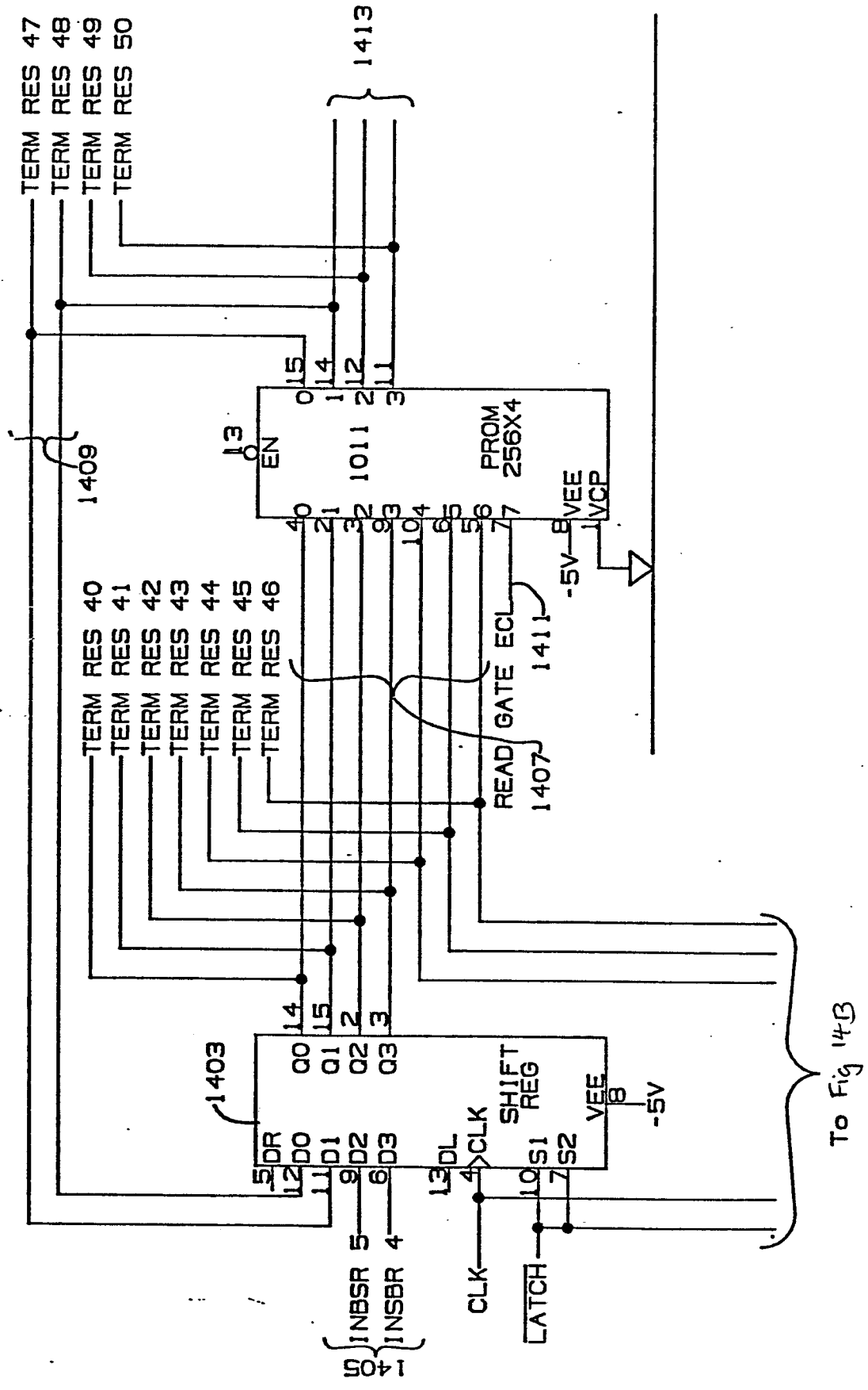
Fig.14A Implementation of Encoding and Decoding
