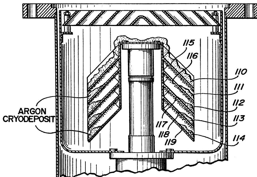
FIG. 3 PRIOR ART
