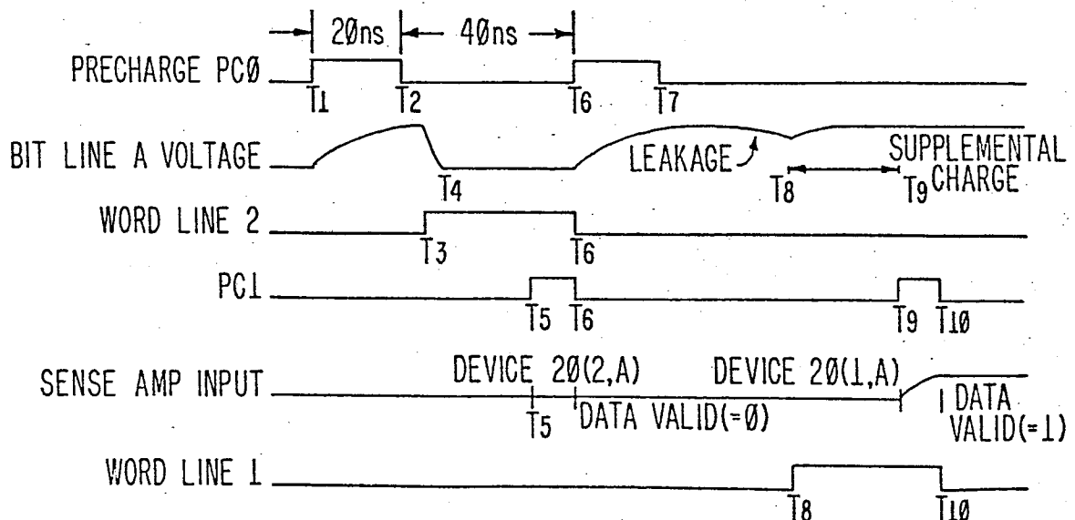
FIG. 3 TIMING DIAGRAM
