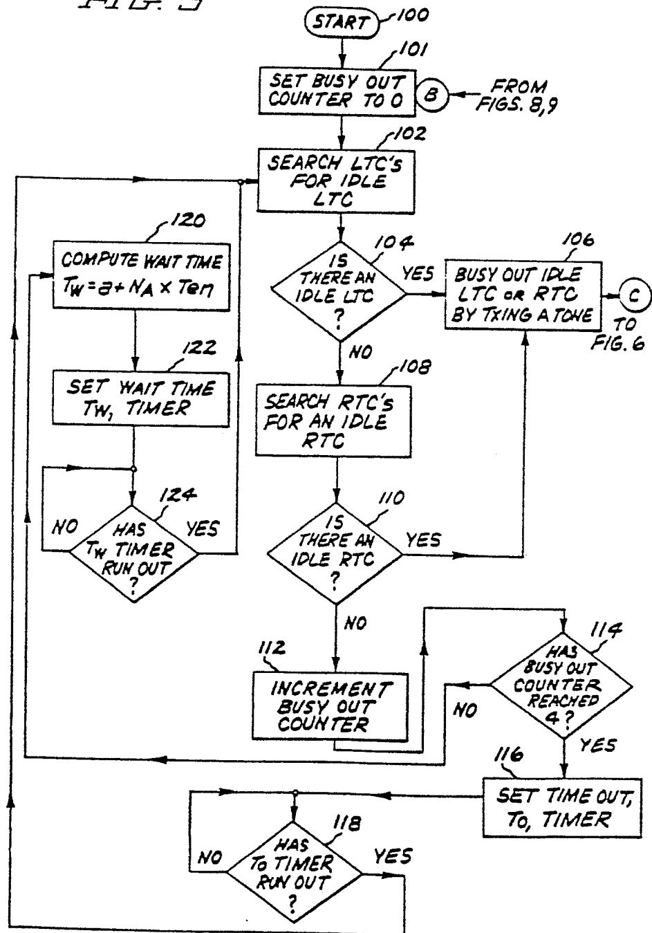
FIG. 5 START UP ROUTINE
