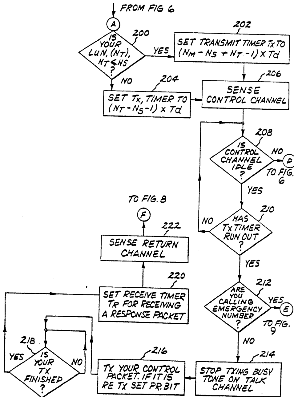
CONTROL PACKET TRANSMIT ROUTINE FIG. 7
