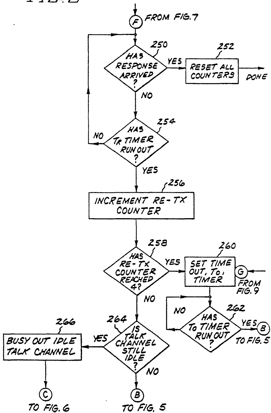
CONTROL PACKET RECEIVE ROUTINE FIG. 8
