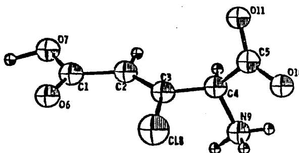
Figure 1 - A computer generated perspective drawing of R-(Z)-4-amino-3-chloro-2-pentenedioic acid showing the correct absolute configuration.
