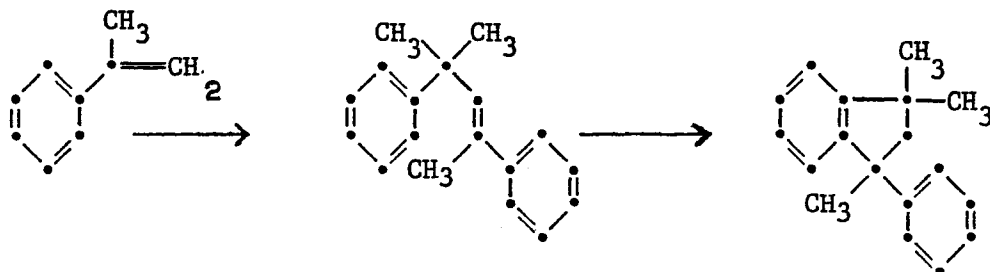
\alpha -Methylstyrol
