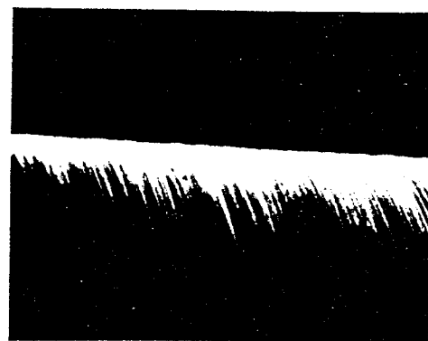
3% PALM OIL +0.2% n-BUTYLTHIOACETIC ACID
