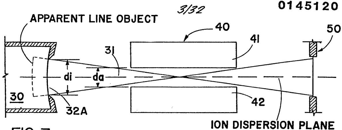
FIG. 7 (PRIOR ART)
