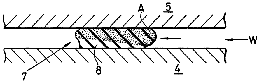
FIG. 4 PRIOR ART
