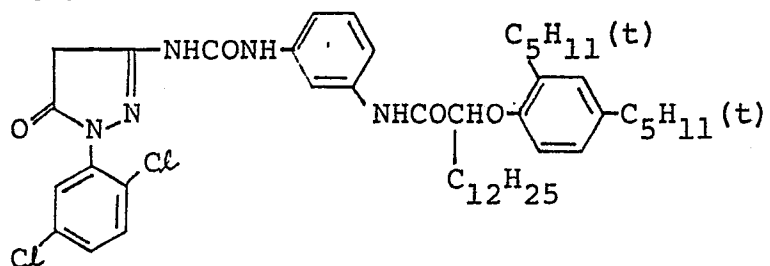
Coupler [C]
