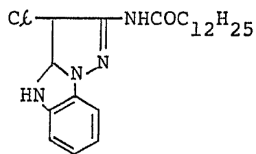
Coupler [D]
