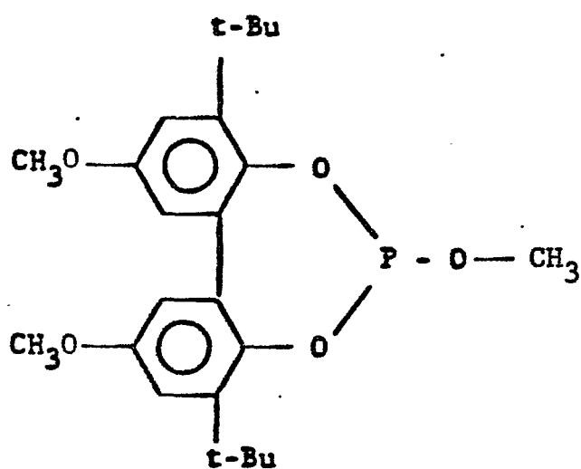
methyl [3,3'-di-t-butyl-5,5'-dimethoxy-1,1'-biphenyl-2,2'-diyl] phosphite
