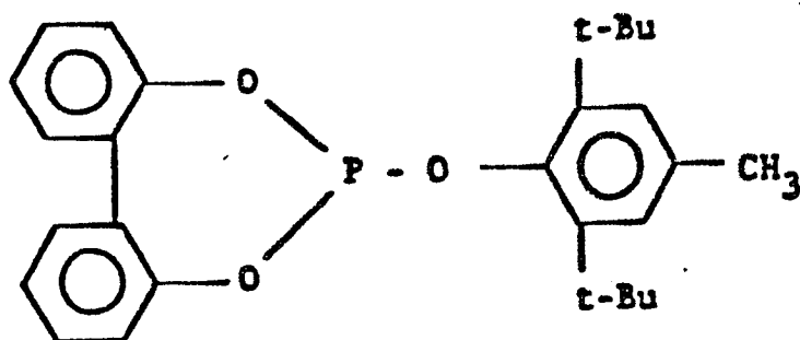
1,1'-biphenyl-2,2'-diyl-(2,6-di-t-butyl-4-methylphenyl) phosphite
