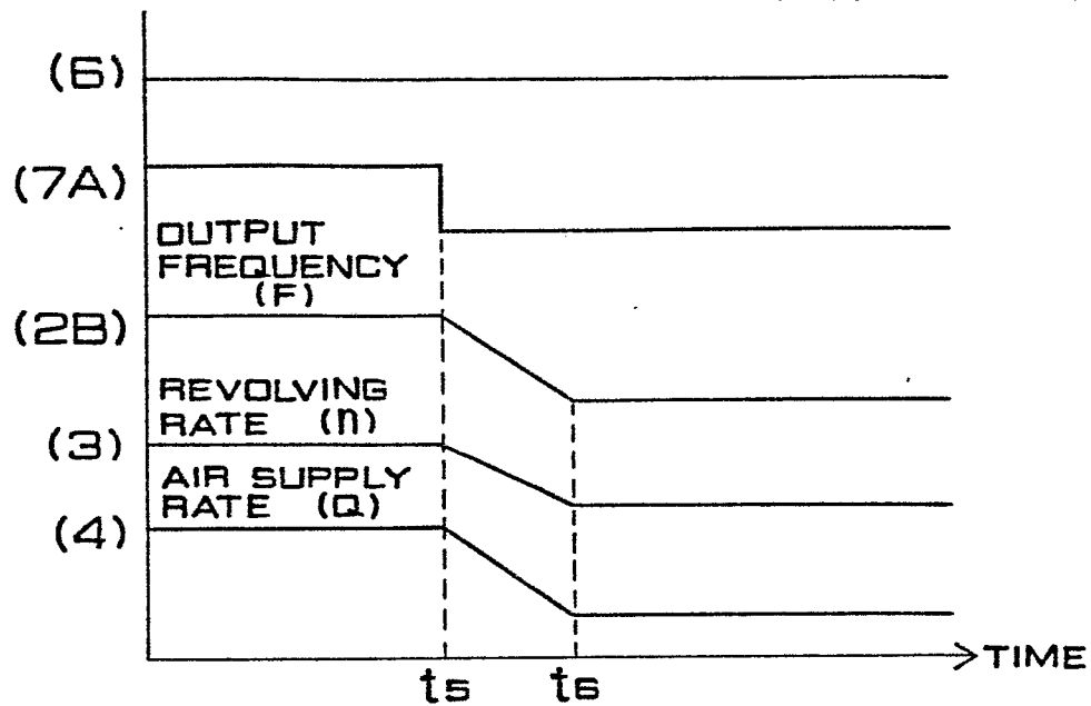
FIG. 3 (PRIOR ART)
