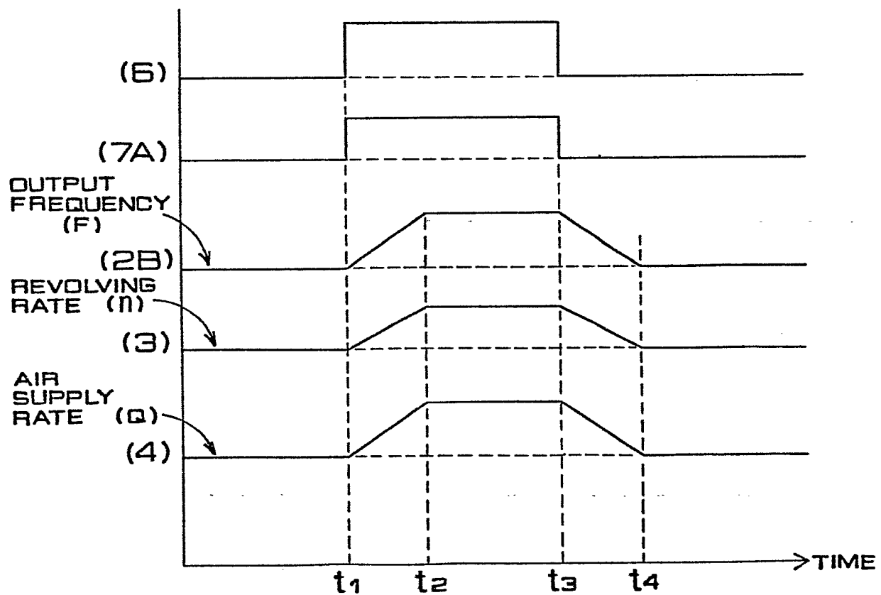
FIG. 2 (PRIOR ART)
