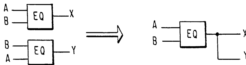
FIG. 5a ELIMINATE COMMON TERMS
