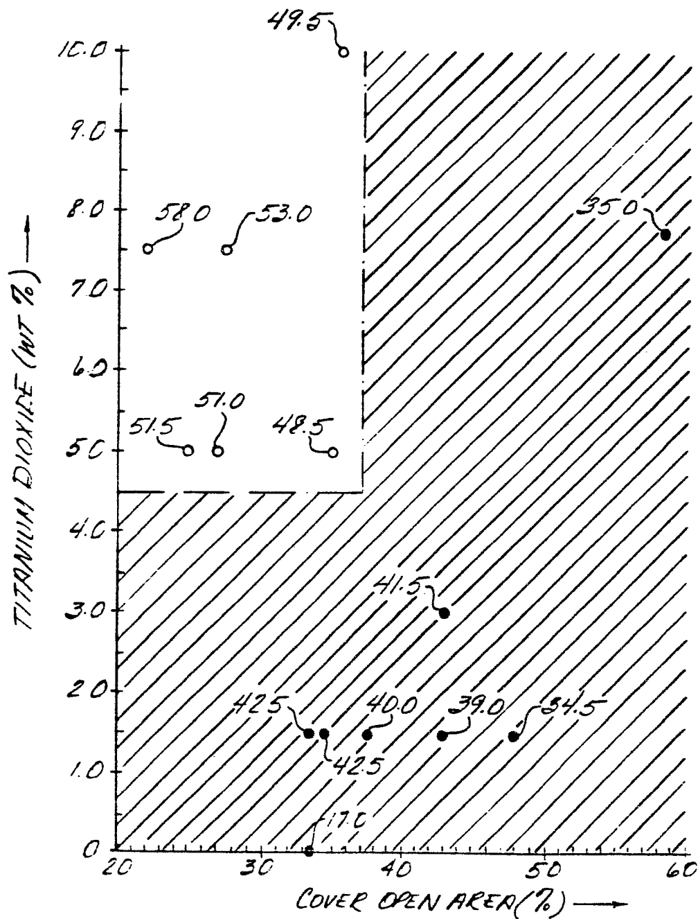
FIG. 7 TITANIUM DIOXIDE CONTENT VS. OPEN AREA (BRIGHTNESS AS PARAMETER)
