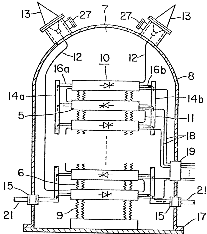
FIG. 1 PRIOR ART
