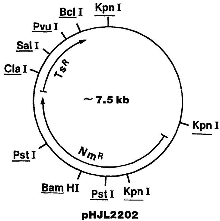
FIG.3 Restriction Site and Functional Map of Plasmids pHJL2202 and pHJL2203
