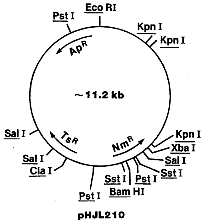
FIG. 6 Restriction Site and Functional Map of Plasmids pHJL210 and pHJL211
