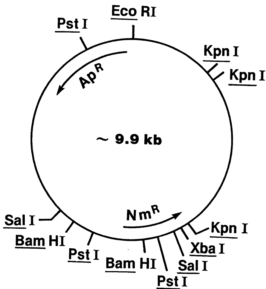
FIG. 4 Restriction Site and Functional Map of Plasmid pHJL201
