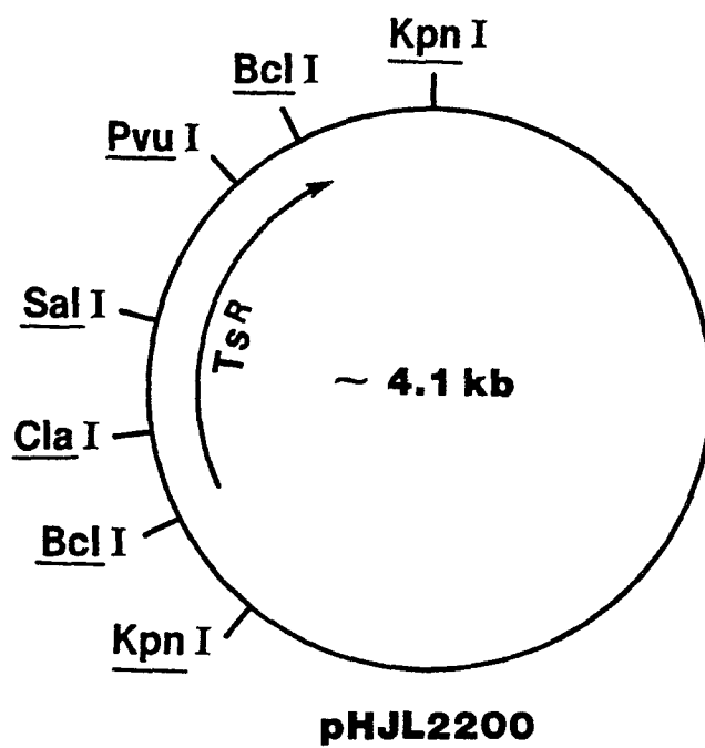
FIG.2 Restriction Site and Functional Map of Plasmids pHJL2200 and pHJL2201
