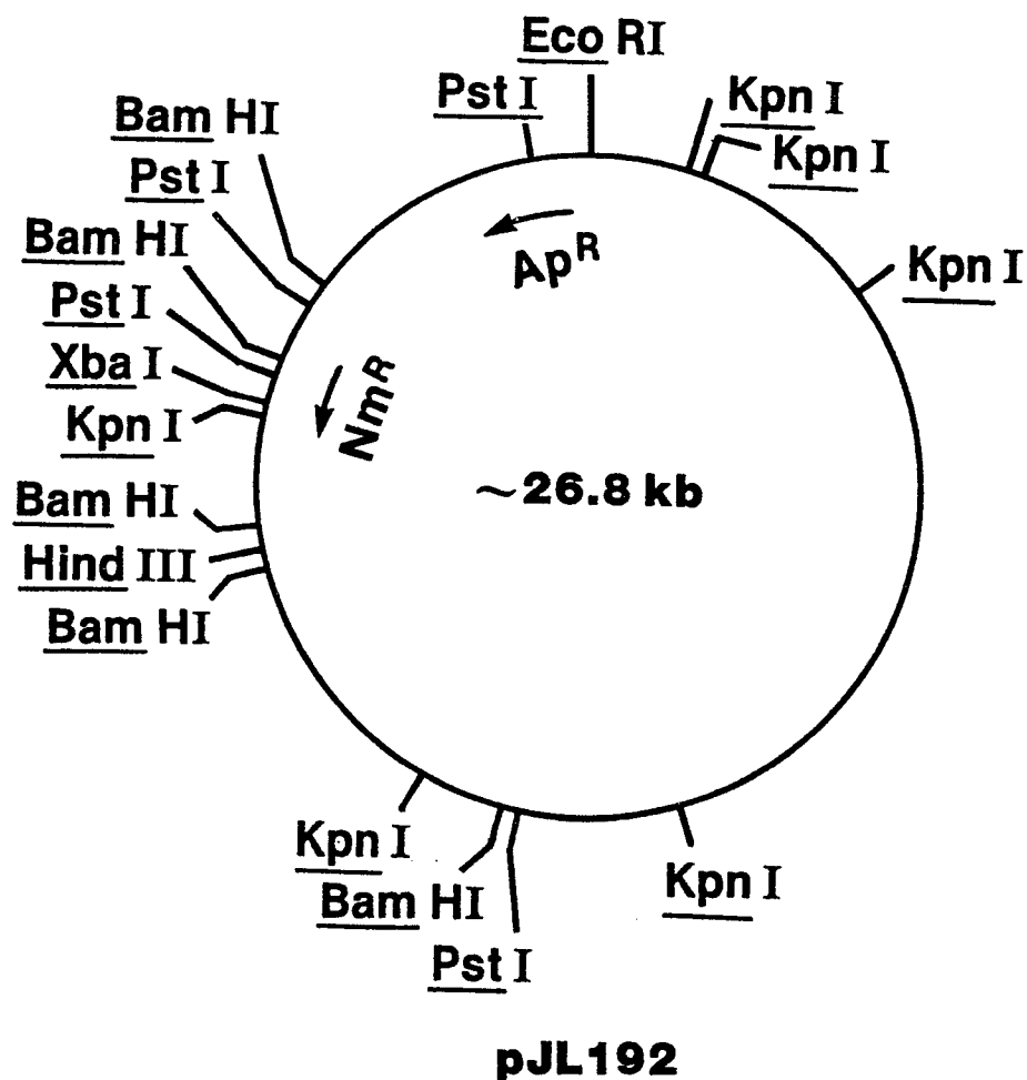
FIG. I Restriction Site Map of Plasmid pJL192.
