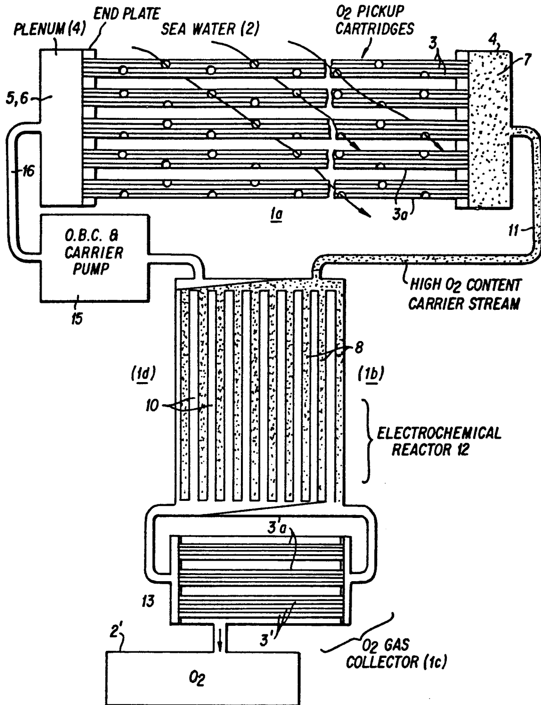
FIG. 4 O 2 EXTRACTION FLUID SYSTEM
