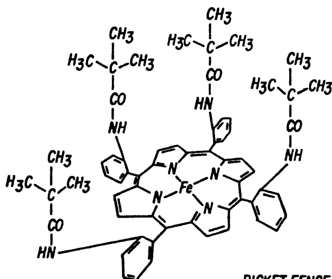
FIG. 17A PICKET FENCE PORPHYRIN SHOWN WITH IRON IN CENTER
