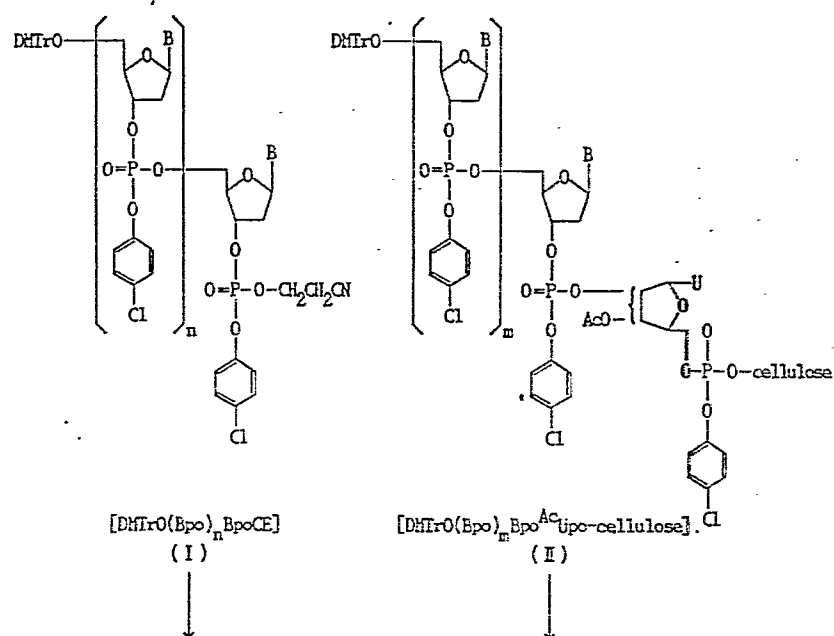
Fig. 1 Building up of oligonucleotides from smaller units by successive coupling reactions (1/4)
