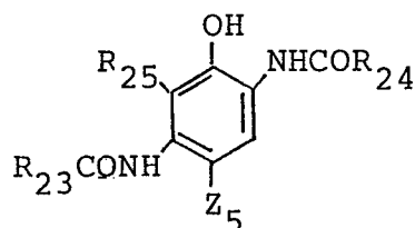
Formula [IX]
