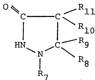
Formula [IV]
