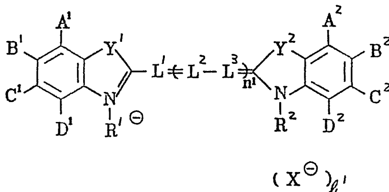
Formula [VII]
