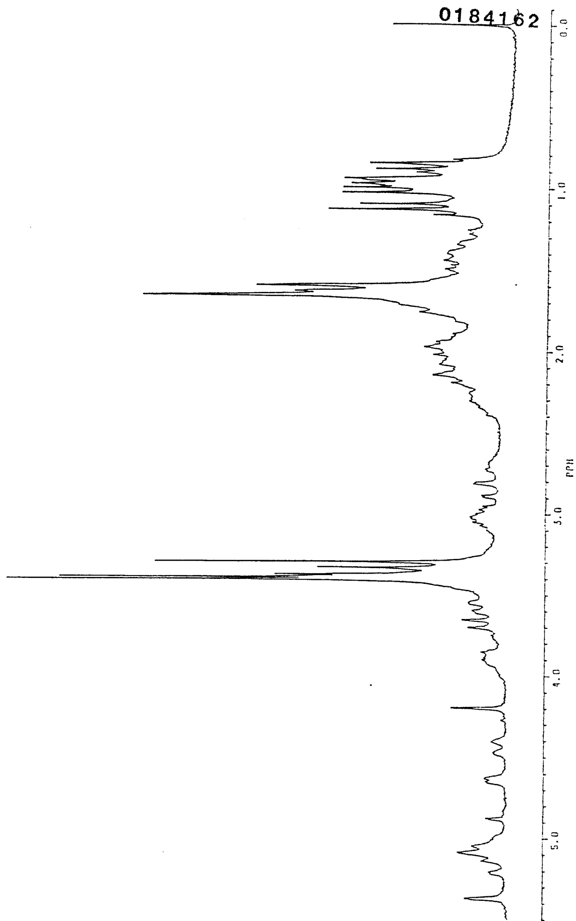
Figure 10 ^1\text{H} Nuclear Magnetic Resonance Spectrum of FR-900523 Substance in \text{CDCl}_3
