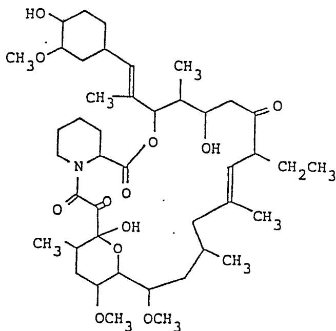
17-Ethyl-1,14-dihydroxy-12-[2-(4-hydroxy-3-methoxycyclohexyl)-1-methylvinyl]-23,25-dimethoxy-13,19,21,27-tetramethyl-11,28-dioxa-4-azatricyclo-[22.3.1.0 4,9 ]octacos-18-ene-2,3,10,16-tetraone
