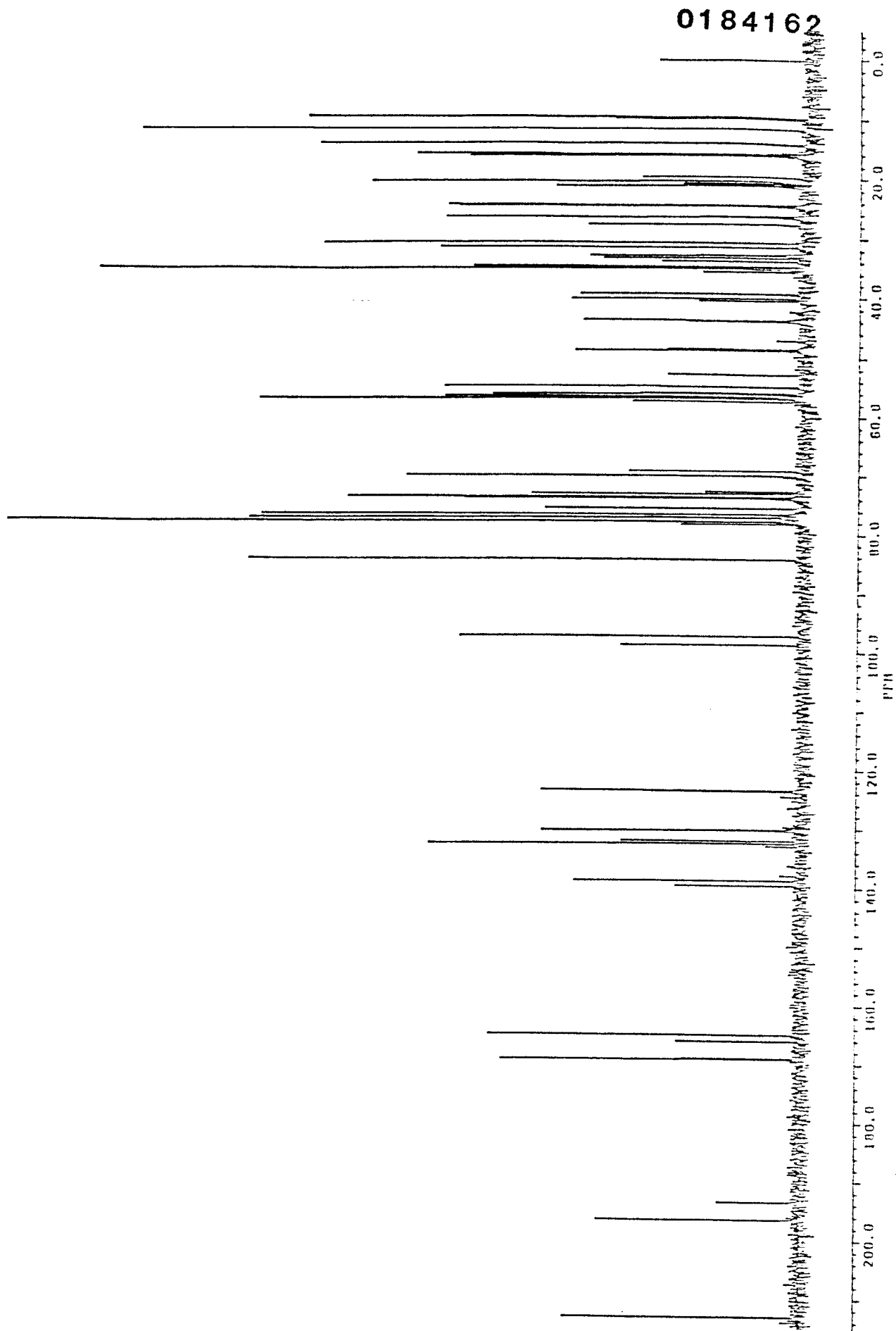
Figure 7 ^{13}\text{C} Nuclear Magnetic Resonance Spectrum of FR-900520 Substance in \text{CDCl}_3
