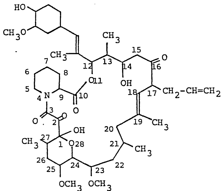
17-Allyl-1,14-dihydroxy-12-[2-(4-hydroxy-3-methoxycyclohexyl)-1-methylvinyl]-23,25-dimethoxy-13,19,21,27-tetramethyl-11,28-dioxo-4-azatricyclo[22.3.1.0 4,9 ]octacos-18-ene-2,3,10,16-tetraone
